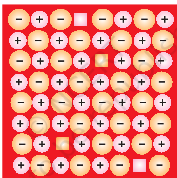
Fig. 1.30: Schottky defects
