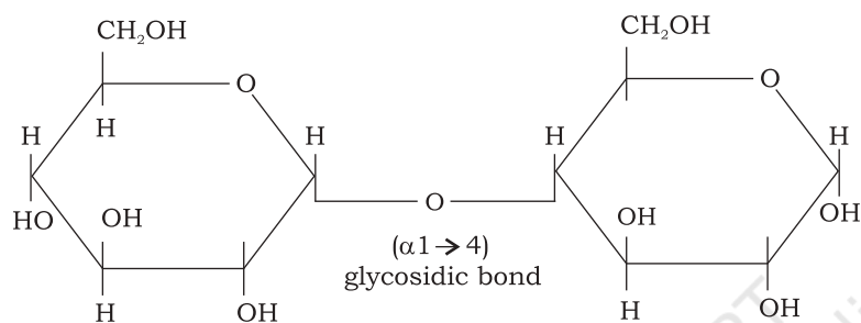
Fig. 3.6: Formation of maltose from two molecules of \alpha D-glucose
