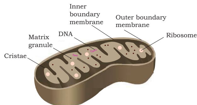
Fig. 2.9: Longitudinal section of mitochondria showing internal structure
