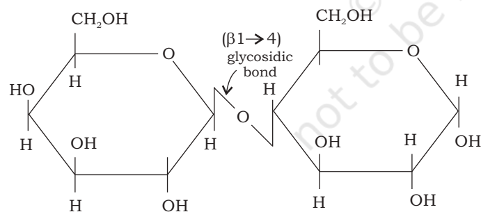
Fig. 3.7: Structure of lactose
