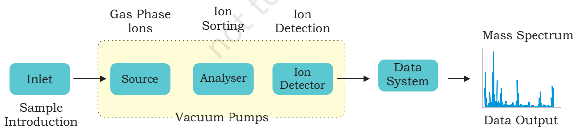
Fig. 12.14: Mass spectrometer
