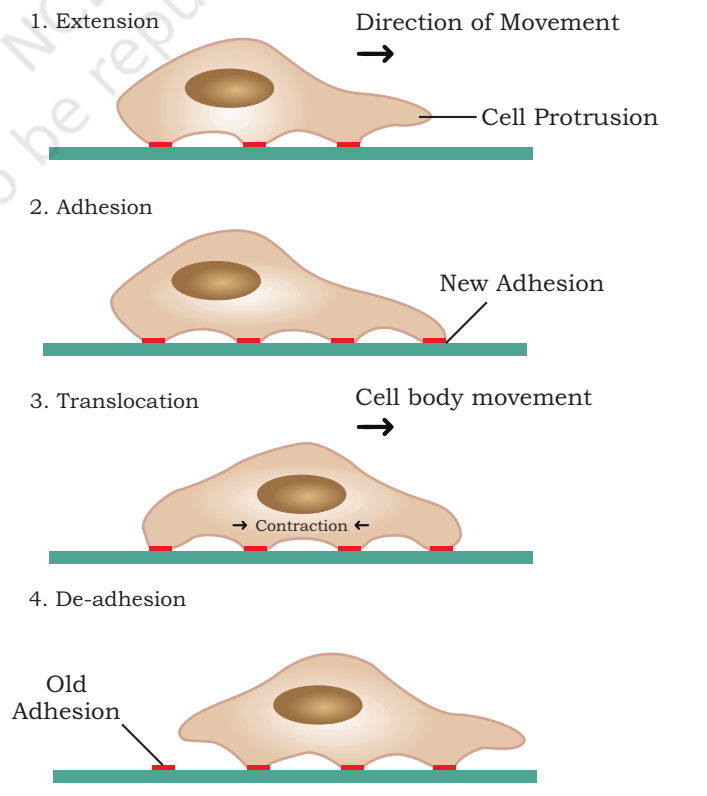
Fig. 5.21: Diagrammatic representation of the steps involved in cell migration
