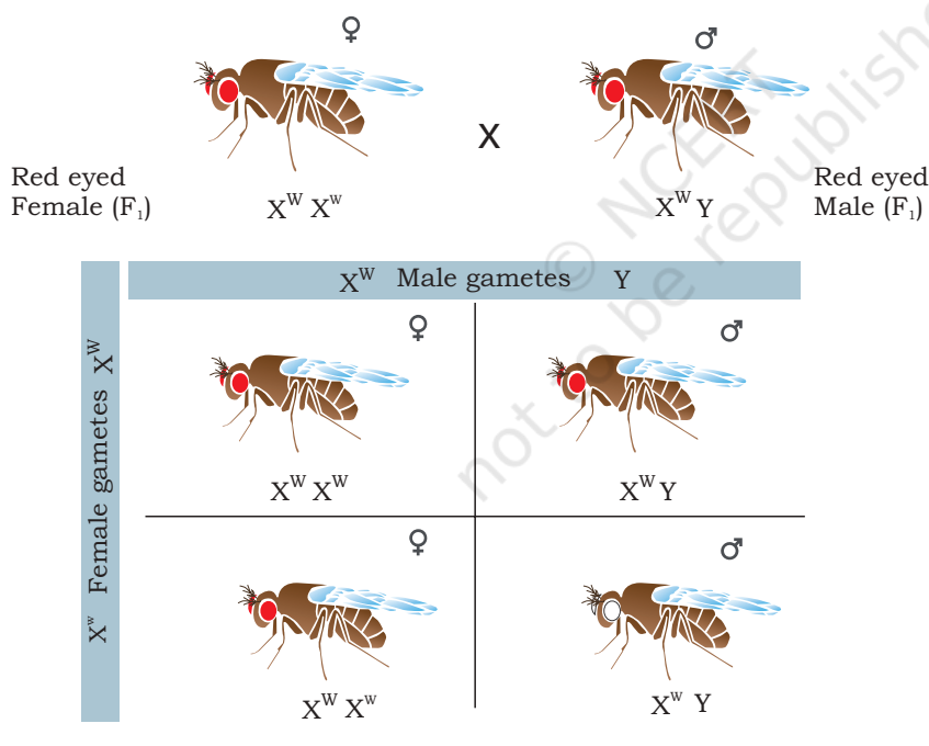
Fig. 6.11: Sex linkage in Drosophila
