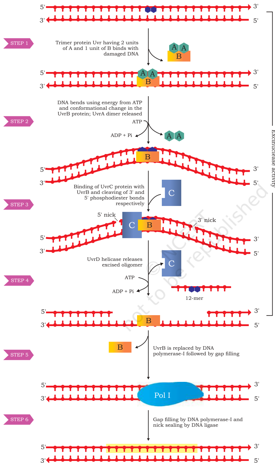
Fig. 7.36: Nucleotide excision repair
