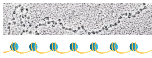
Fig. 7.5: Beads on string structure of chromatin
