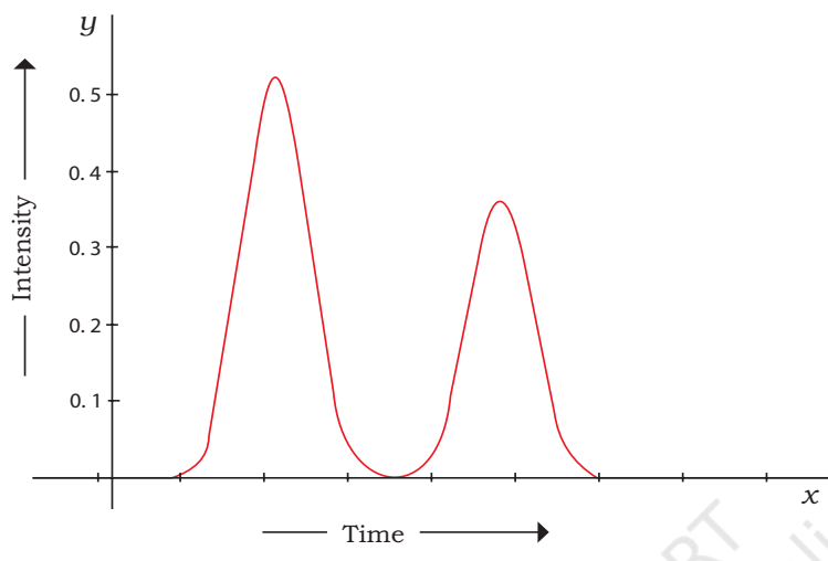
Fig. 12.10: HPLC chromatogram
