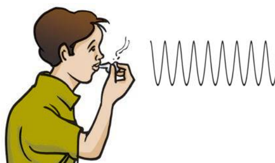
Fig. 13.18 : Frequency determines the pitch of a sound
