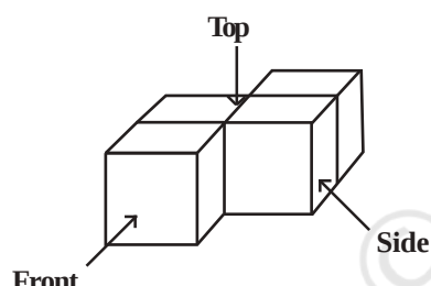
Solid made of four cubes
