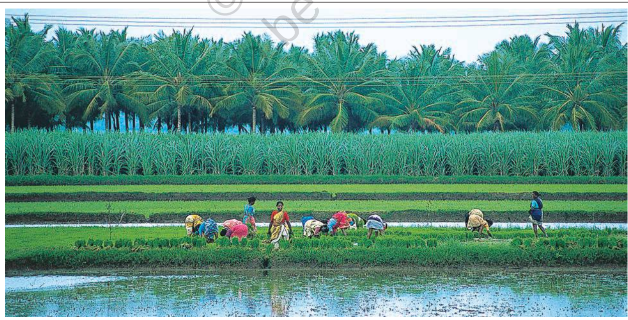
Figure 6.6 : Plains
