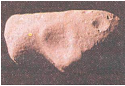
Figure 1.5 : Asteroid
